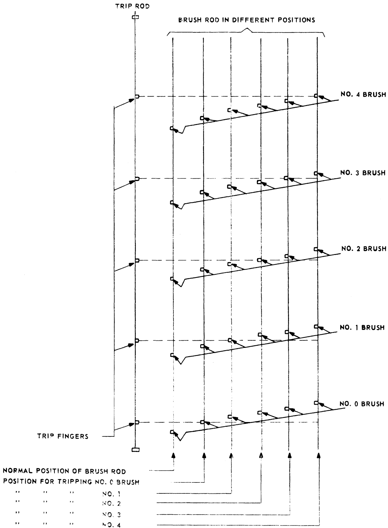
Figure 5-7 Brush Selection
