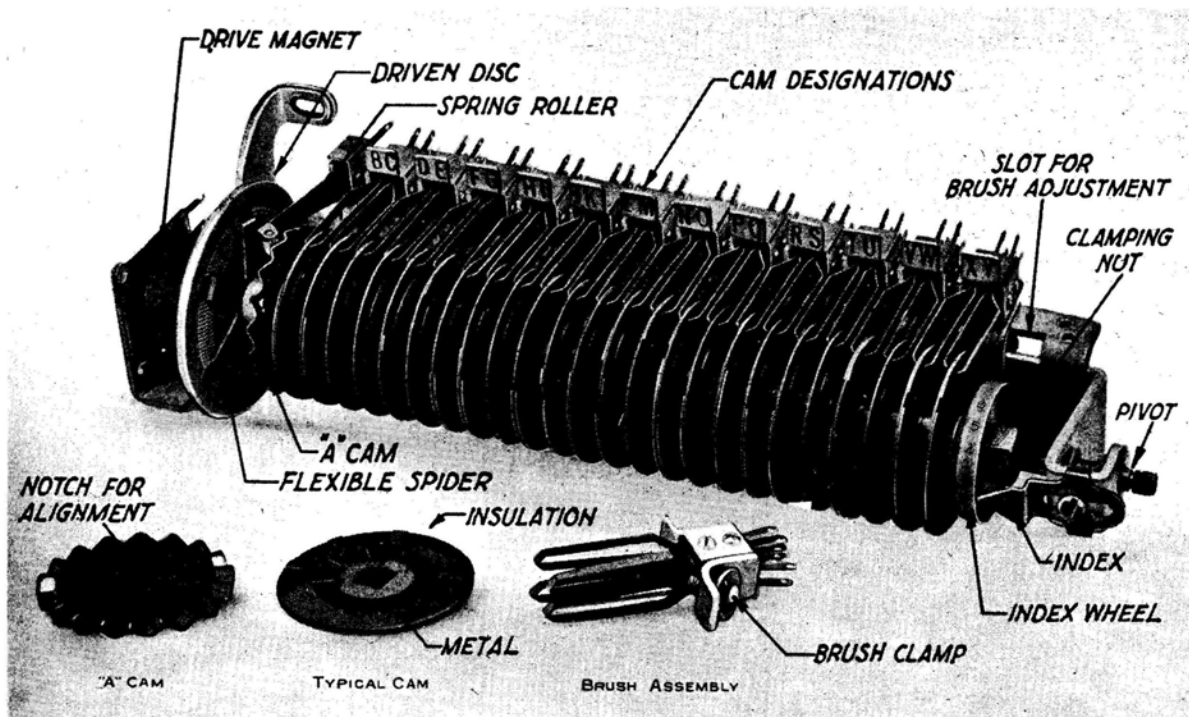
Figure 5-8 Sequence Switch
